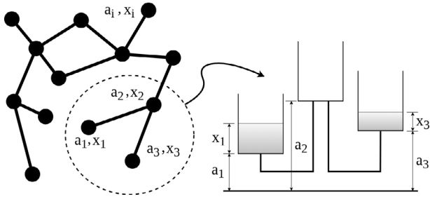
Fig. 1. Graph structure and the connected water tanks interpretation.
