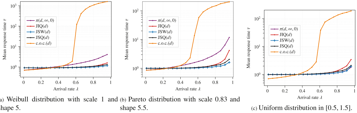
Fig. 9. The mean response time as a function of normalized arrival rate \lambda for the policies JIQ(d) , JSW(d) , JSQ(d) , c.o.c.(d) with respect to the \pi(d, \infty, 0) policy, for the number of servers N = 20 and the number of replicas d = 4 .
