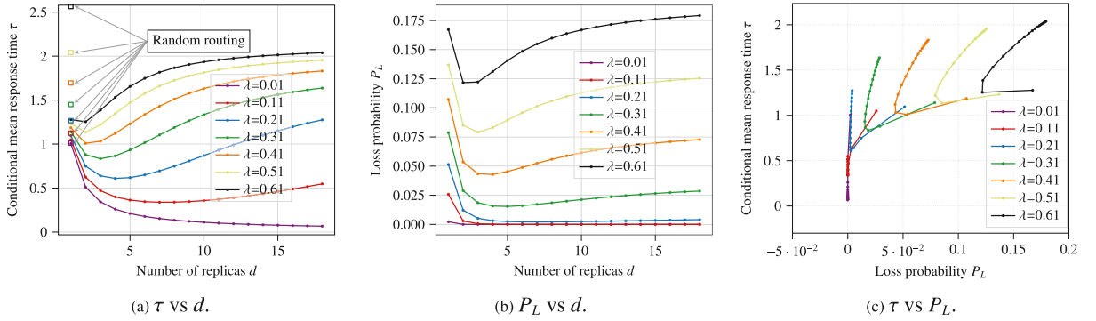
Fig. 2. We plot the conditional mean response time \tau and the loss probability P_L for the policy \pi(d, T, T) as a function of the number of replicas d , for a fixed discard threshold T = 1.5 , the number of servers N = 20 , service rate \mu = 1 , and different values of arrival rate \lambda \in \{0.01, 0.11, \dots, 0.61\} .
