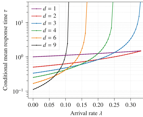
(a) \tau vs arrival rate \lambda for discard threshold T_2 = \infty .
