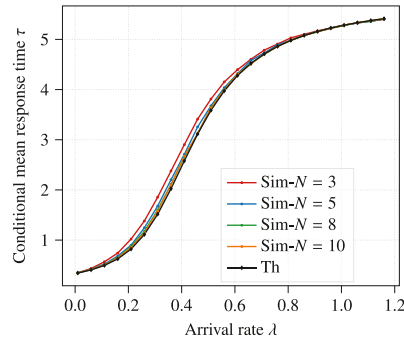
Fig. B.10. For the policy \pi(d, T, T) with fixed thresholds T_1 = T_2 = 5 , number of replicas d = 3 , service rate \mu = 1 , conditional mean response time \tau as function of arrival rate \lambda for different values of servers N \in \{3, 5, 8, 10\} .
