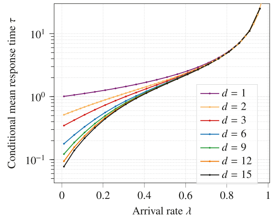
(b) \tau vs arrival rate \lambda for discard threshold T_2 = 0 .
