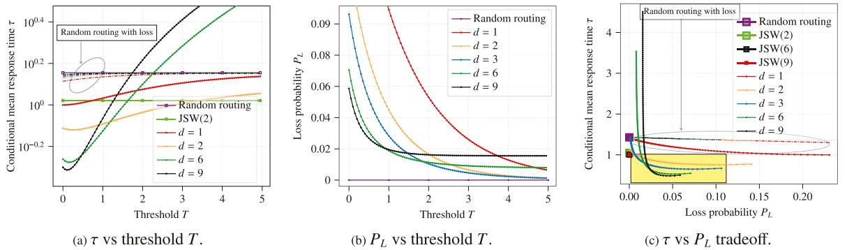
Fig. 3. We plot the conditional mean response time \tau and the loss probability P_L for the policy \pi(d, T, T) as a function of discard threshold T , for the number of servers N = 20 , arrival rate \lambda = 0.3 , service rate \mu = 1 , and for the number of replicas d \in \{1, 2, 3, 6, 9\} .
