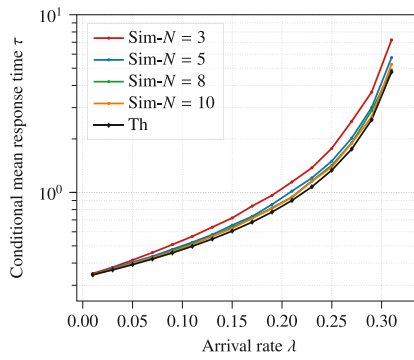
Fig. B.11. For the policy \pi(d, \infty, \infty) with number of replicas d = 3 , service rate \mu = 1 , conditional mean response time \tau as function of arrival rate \lambda for different values of servers N \in \{3, 5, 8, 10\} .
