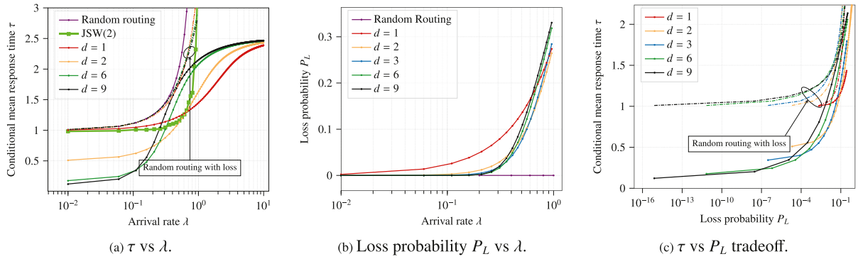
Fig. 5. We plot the conditional mean response time \tau and the loss probability P_L as the normalized arrival rate \lambda increases under policy \pi(d, T, T) for the number of servers N = 20 , discard threshold T = 1.5 , service rate \mu = 1 , and the number of replicas d \in \{1, 2, 3, 6, 9\} .
