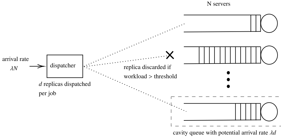
Fig. 1. The N server system under \pi(d, T_1, T_2) policy with a job arrival rate \lambda N . The dispatcher dispatches d replicas per job and the potential arrival rate at any cavity queue is \lambda d .
