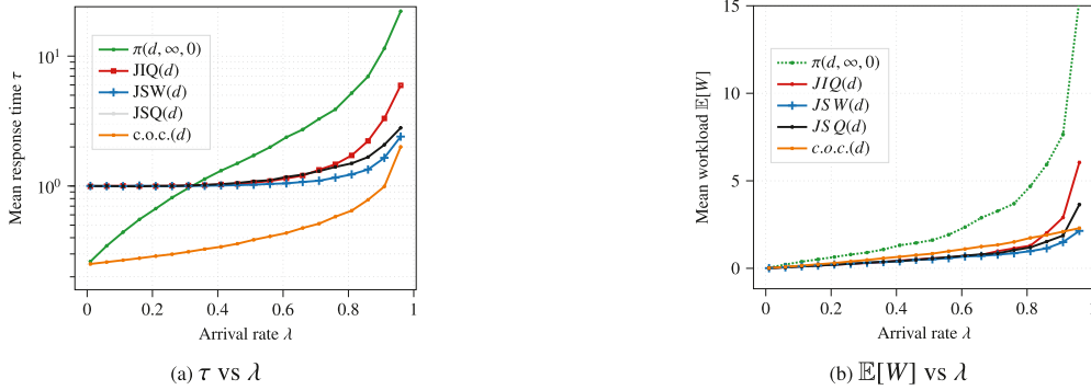
Fig. 8. The mean response time \tau and the mean workload \mathbb{E}[W] at the cavity queue as a function of normalized arrival rate \lambda for the policies \pi(d, \infty, 0) , JIQ(d) , JSW(d) , JSQ(d) , c.o.c.(d) for exponential service distribution of rate \mu = 1 , the number of servers N = 20 and the number of replicas d = 4 .
