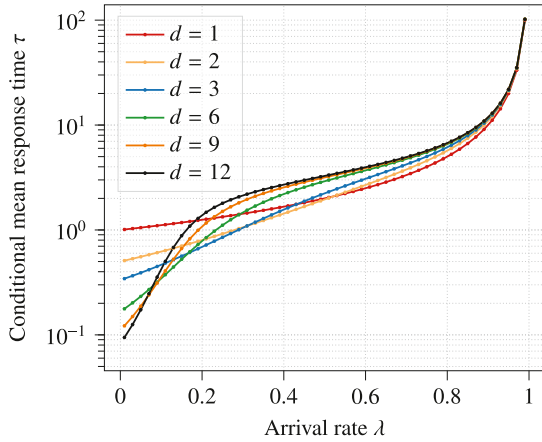
(a) \tau vs arrival rate \lambda for discard threshold T_2 = 2 .
