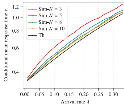
Fig. B.12. For the policy \pi(d, \infty, 0) with number of replicas d = 3 , service rate \mu = 1 , conditional mean response time \tau as function of arrival rate \lambda for different values of servers N \in \{3, 5, 8, 10\} .
