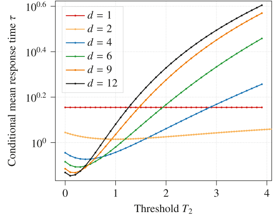
(b) \tau vs discard threshold T_2 for arrival rate \lambda = 0.3
