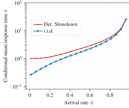
Fig. E.13. For the deterministic slowdown with slowdown factor s = 1 and i.i.d. service times under \pi(d, \infty, 0) policy with number of replicas d = 4 , service rate \mu = 1 and number of servers N = 20 , conditional mean response time \tau as function of arrival rate \lambda .
