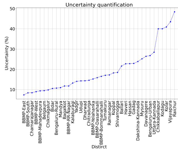
Figure 5: Uncertainty quantification for the validation period in each unit of Karnataka. More than one-half of the units have a root mean squared error of less than 20%. Five districts have errors between 40-50% which are due to the sudden change in trends in the reported cases not captured by the model.
