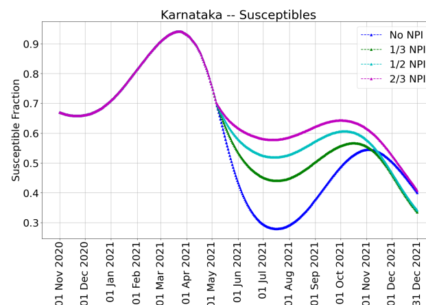
Figure 7: The evolution of susceptible fraction in the state of Karnataka over time. These plots are for the vaccination policy that allocates 167000 vaccine doses per day proportional to each unit's population. Observe that the susceptible fraction increase during the period August-November 2021 due to antibody waning.
