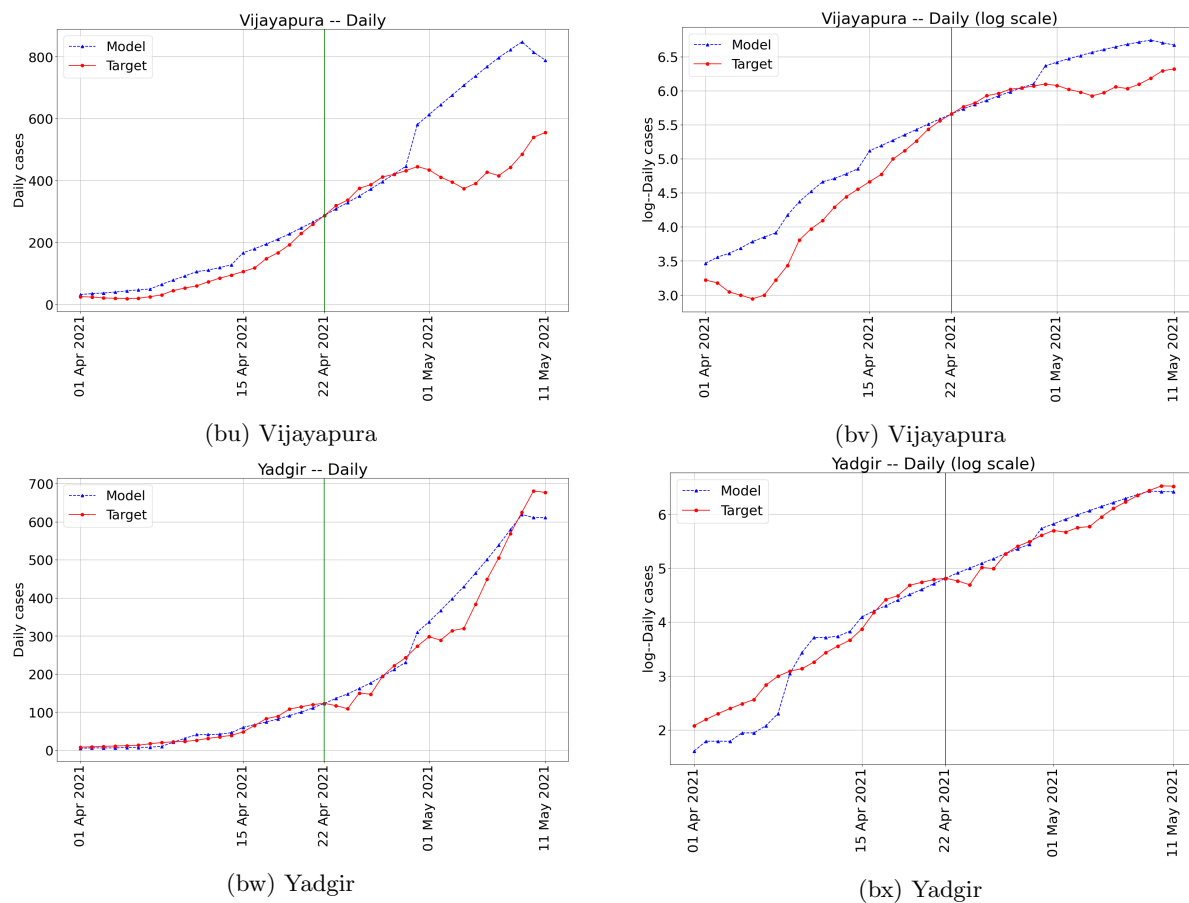
Figure 13: Validation plots for each unit. Calibration has been performed from 08–22 April 2021 and validated during 23 April – 11 May 2021. The vertical line separates the calibration and the validation phases.
