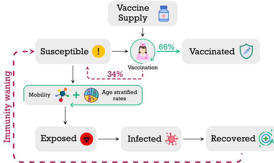
Figure 2: Compartments, disease progression, vaccination, and immunity waning (antibody decay) components of the model.
