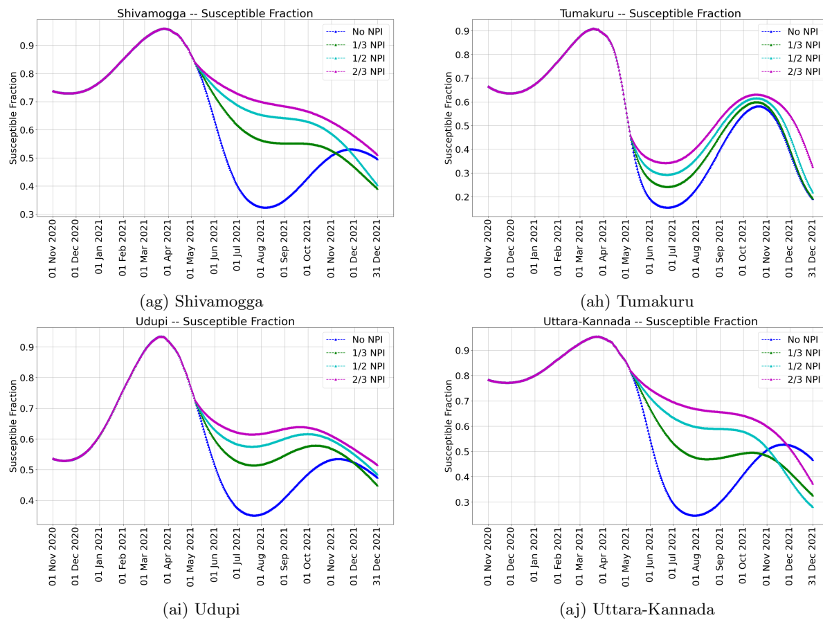
Figure 12: Susceptible fractions in each unit for various NPI intensities. Vaccination capacity is 167000 per day allocated in proportion to population in the units.
