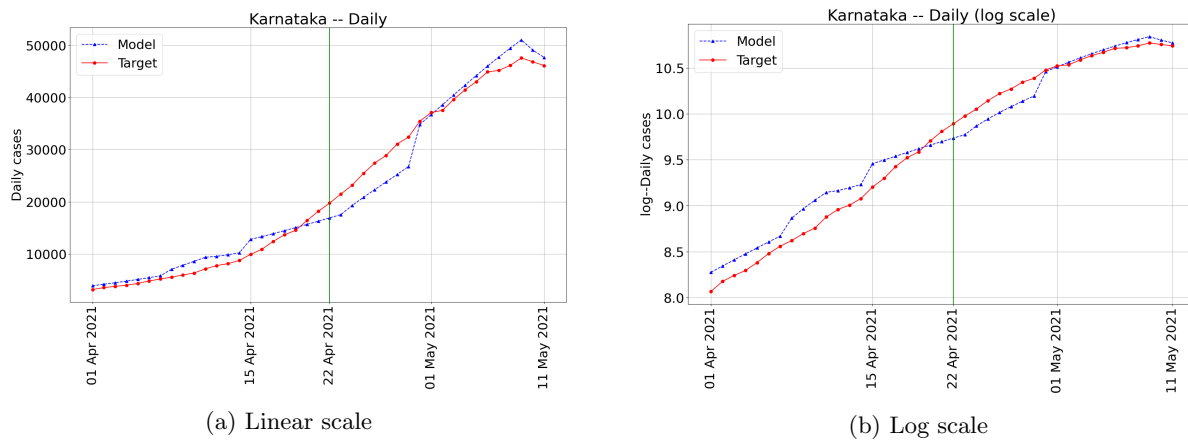
Figure 4: Validation plots for the state of Karnataka. The vertical line in both plots separates the calibration and the validation periods. The root mean squared error during the validation period is at most 9% for the state of Karnataka.
