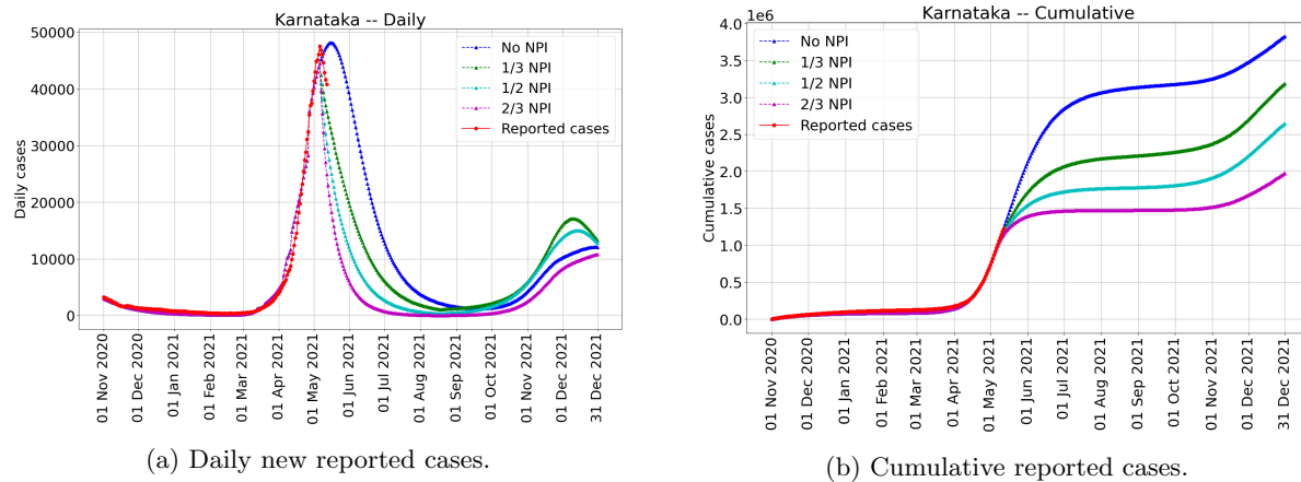
Figure 6: The projected number of new infections for the state of Karnataka under various NPIs. These projections are for the vaccination policy that allocates 167000 vaccine doses per day proportional to each unit's population. Uncertainty bands are not indicated to reduce clutter. Recall the 9% root mean squared error for a two-week ahead projection. The left figure is for the daily new reported cases, and the right figure provides the cumulative reported cases.
