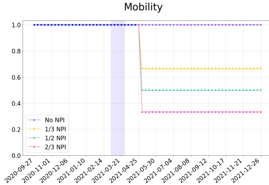
Figure 3: Mobility scenarios considered for the simulation experiment design. The purple band indicates a period when the mobility matrix is (1 - \varepsilon)I + \varepsilon J . The mobility is I at all other times.
