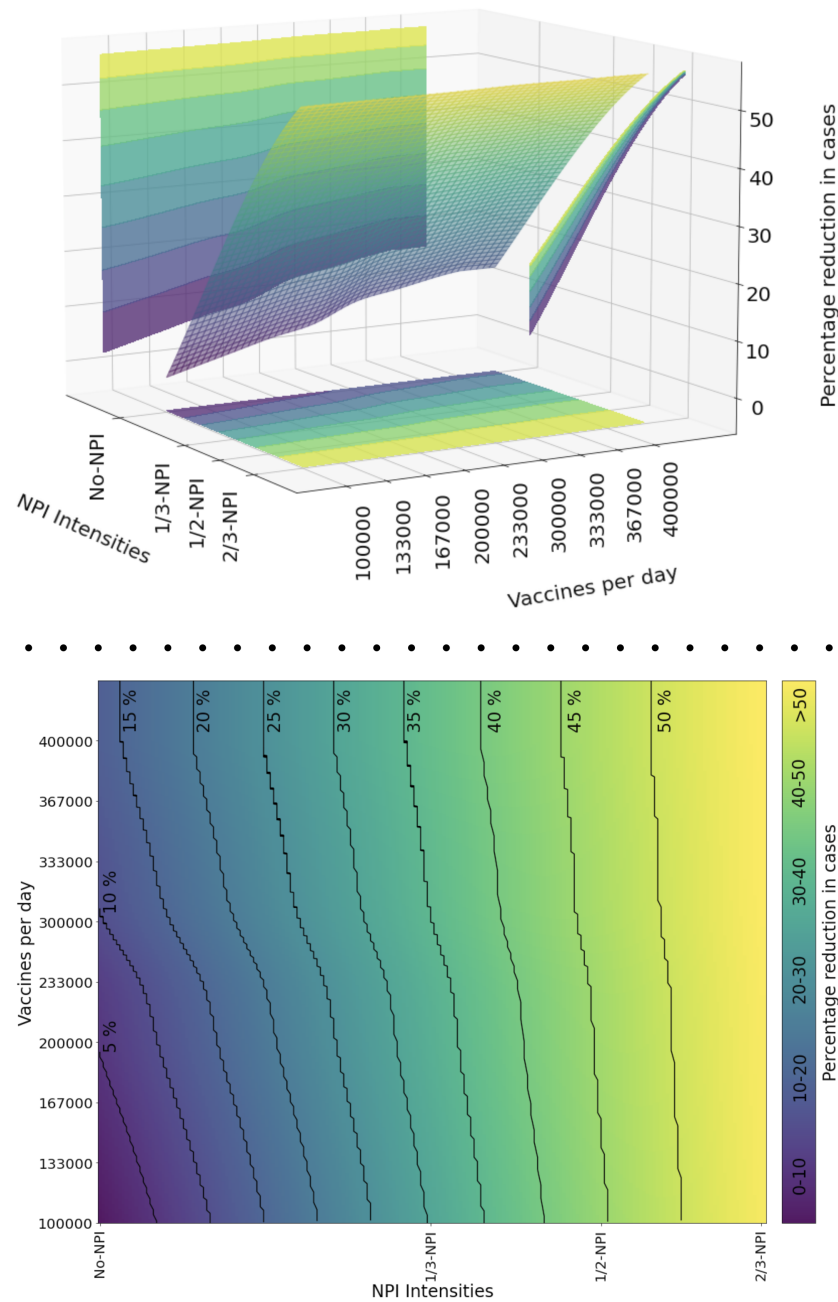
Figure 8: Surface plot (top figure) and contour plot (bottom figure) summarising the reduction in the number of model-projected cases on 31 August 2021 for varying daily vaccination budgets and NPI intensities. The surface plot and the contours are based on linear interpolation from the data points in Table 3.
