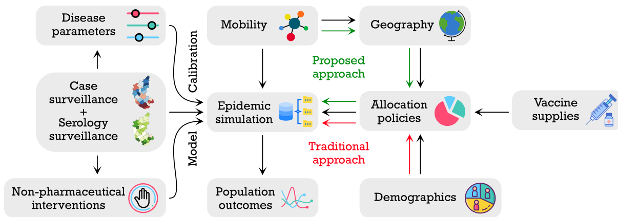
Figure 1: Datasets for our epidemic simulator. The epidemic simulator takes data from several sources. Disease parameters come from the current state of knowledge of how COVID-19 affects an infected individual. Case surveillance data include tests, reported cases, discharges, and deaths. Serosurveillance data comes from a state-wide survey done in September 2020 during the first peak. The timings and the duration of the NPIs are based on when they come into effect in the state. A mobility model captures the spread of infection in the units before the April 2021 resurgence. Karnataka’s actual geography enables better visualisation of the simulation outcomes. Demographic data for the units are taken from the 2011 census and extrapolated to 2020. Vaccine supply assumptions are based on historical vaccination data. Experimental vaccination allocation policies are based on these data elements. The epidemic simulator takes all these and generates outcomes for a comparative study.
