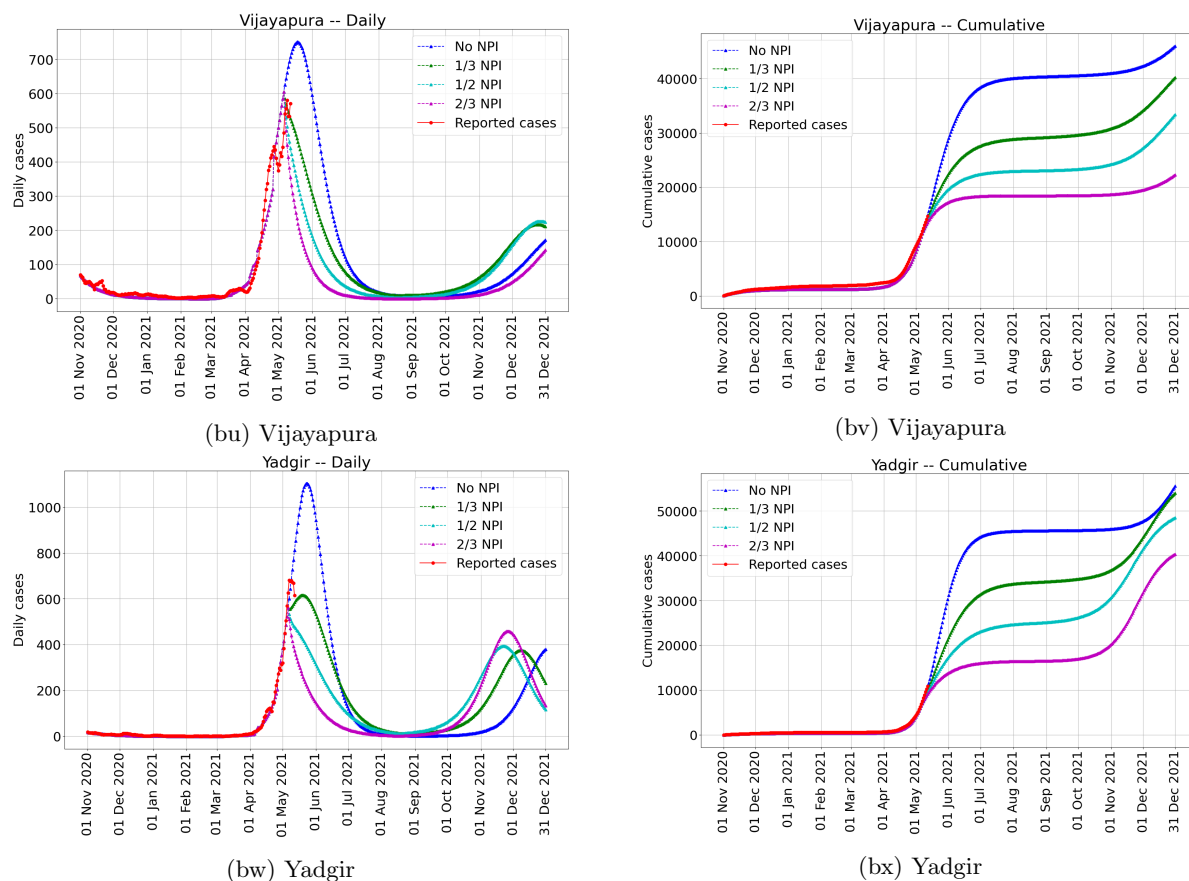
Figure 11: Daily predicted number of cases in each unit until 31 December 2021 for various NPI intensities. Vaccination capacity is 167000 per day allocated in proportion to population in the units.
