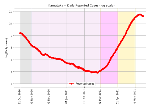
Figure 10: Log plot of the daily infections (averaged over seven days to avoid weekly periodicity issues). The different phases are colour coded. During October 2020, we initialise the simulator. During 01 November 2020 – 28 February 2021, we capture the receding trend. As seen above, both are well-captured by straight lines. During 01 March 2021 – 31 March 2021, we calibrate to re-seed the infections across the units and handle stochasticity. From 01 April 2021 - 01 May 2021, we capture the resurgence and the \lambda_1 associated with it. All projections are from 02 May 2021 onward.
